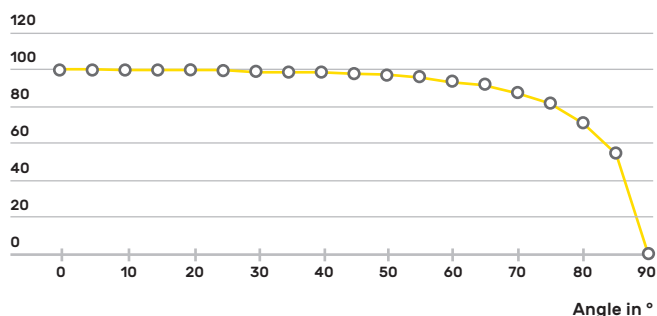
Incident Angle Modifier %
