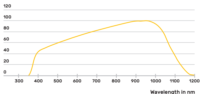
Normalized Spectral Response SR %
