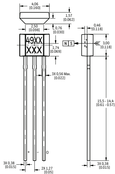
Figure 4. SS490 Series Flat TO-92-Style Mounting and Dimensional Drawings (For reference only: mm/[in].)
